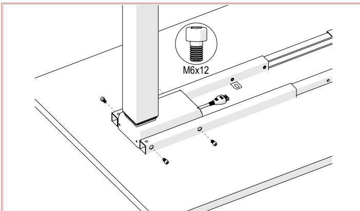
Step 3 Assemble the Top Frame and Leg as illustrated above. Please refer to Torque Guide .
