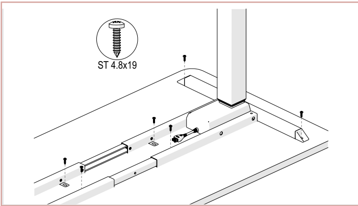
Step 7 Mount the Frame to the Table top and fix the Top Frame as illustrated above. Please refer to Torque Guide .
