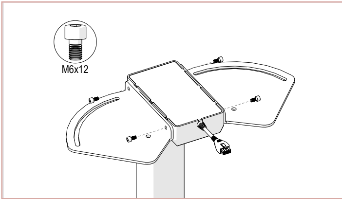
Step 1 Assemble the middle Leg and Bracket as illustrated above. Please refer to Torque Guide .
