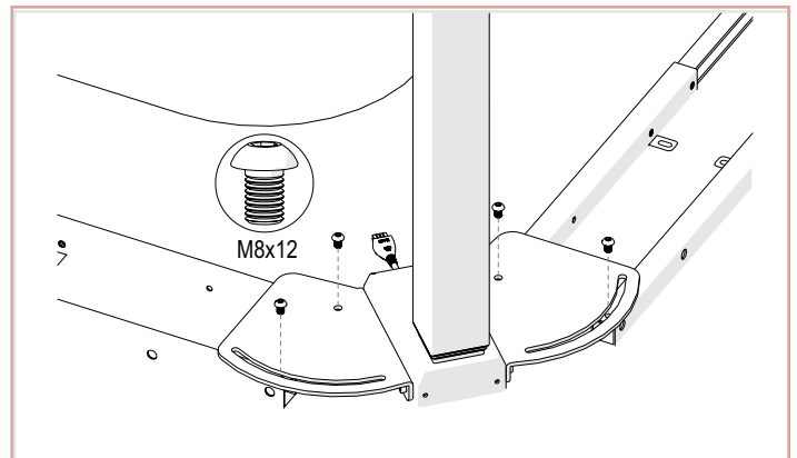
Step 4 Assemble the middle Leg and 3rd Leg Bracket as illustrated above. Please refer to Torque Guide .
