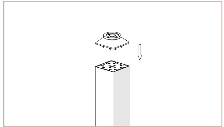
Step 2 Mount the Adjustment Feet to the middle Leg as illustrated above. Please punch in, do not use a hammer.
