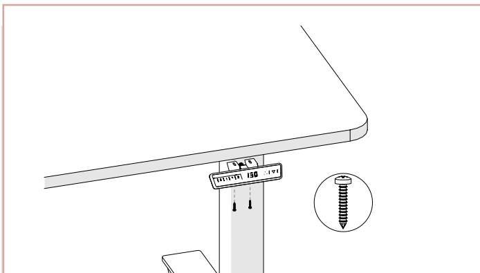
Step 11 Mount the Remote Control to the Table top as illustrated above. Please refer to Screw Part List Select the appropriate feet and the matching screw. Please refer to Torque Guide .
