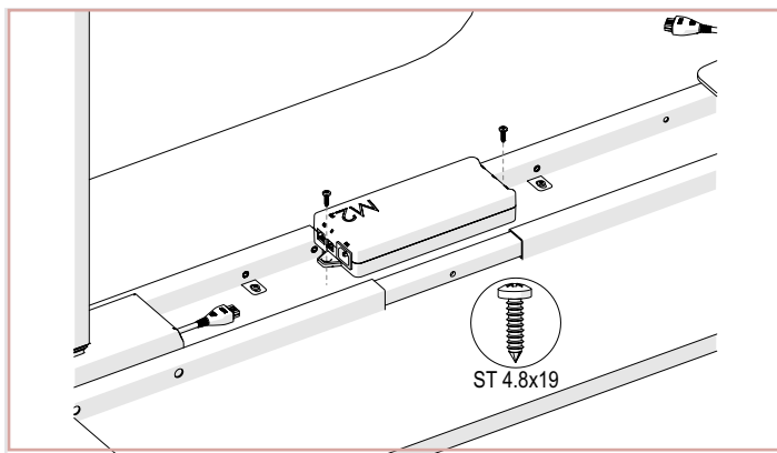
Step 9 Mount the Control Unit as illustrated above. Please refer to Torque Guide .
