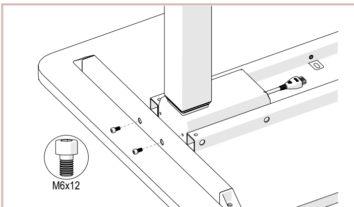
Step 5 Assemble the Leg and End Pipe for both left and right side as illustrated above. Please refer to Torque Guide .
