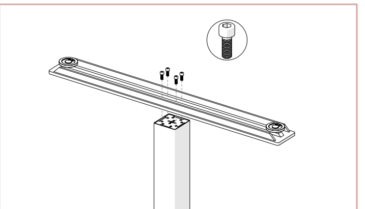
Step 6 Mount the Feet as illustrated above. The smooth side of the plate faces the foot. Please refer to Screw Part List Select the appropriate feet and the matching screw. Please refer to Torque Guide .
